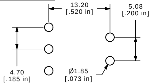
P.C. MOUNTING
