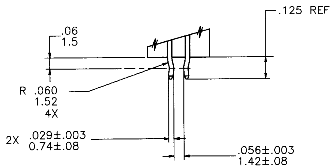
SECTION X-X NOTE 8
