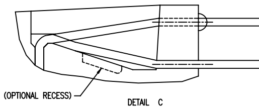
DETAIL C
