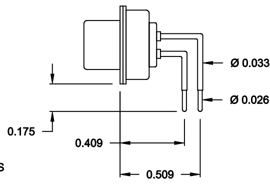
SIGNAL CONTACTS
