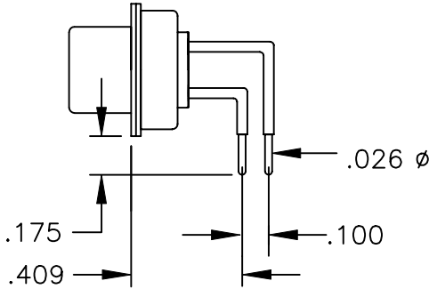
SIGNAL CONTACTS
