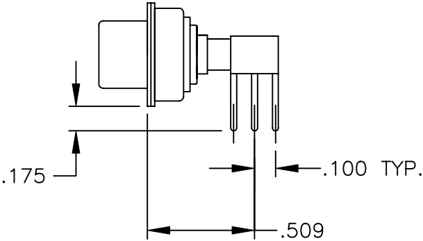
75 OHM COAXIAL CONTACTS
