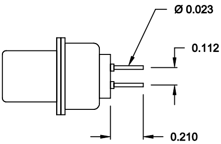
SIGNAL CONTACTS
