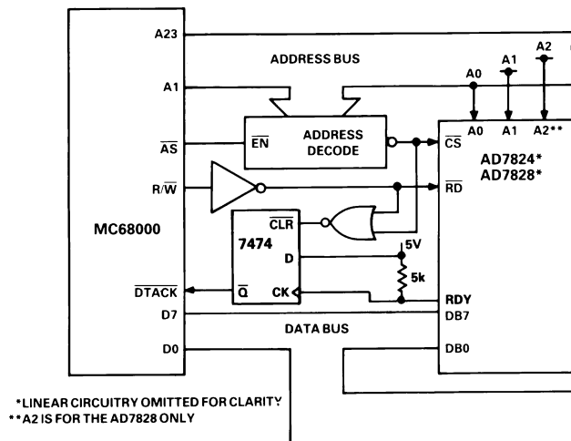
Figure 17. AD7824/AD7828–MC68000 Interface
