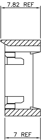
SECTION B-B
