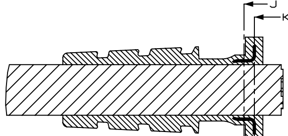
SECTION G-G
