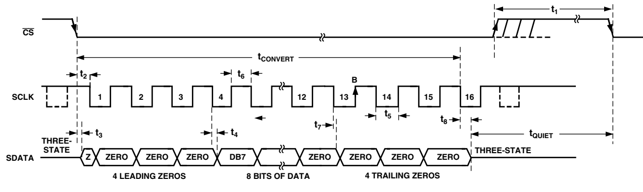
Figure 23. AD7478 Serial Interface Timing Diagram
