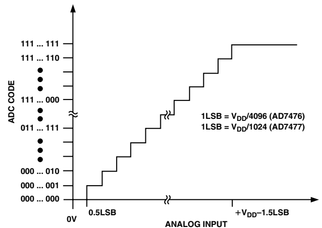
Figure 10. Transfer Characteristic for the AD7476/AD7477
