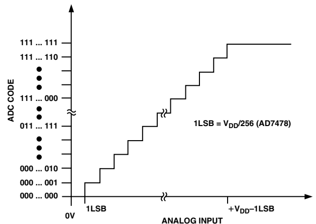
Figure 11. Transfer Characteristic for AD7478
