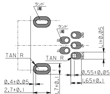
RECOMMENDED P.C.B. PATTERN LAYOUT
