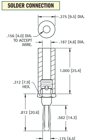
.175 (4.5) Plug
