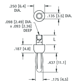
.175 (4.5) Plug
