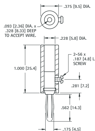
.175 (4.5) Plug
