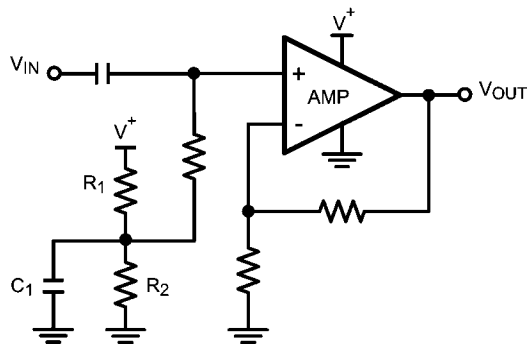
FIGURE 3. Single Supply Virtual Ground
