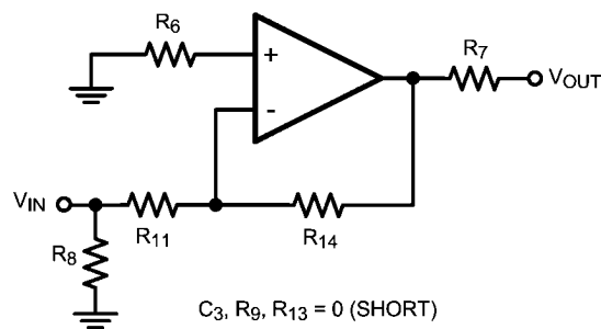
FIGURE 5. Inverting Amplifier
