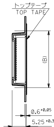
SECT. Z-Z
