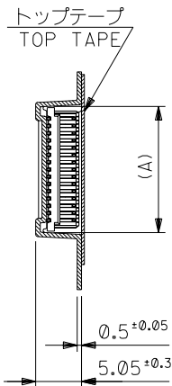
SECT. Y-Y
