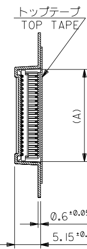
SECT. Z-Z
