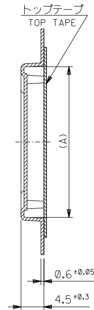
SECT. Z-Z
