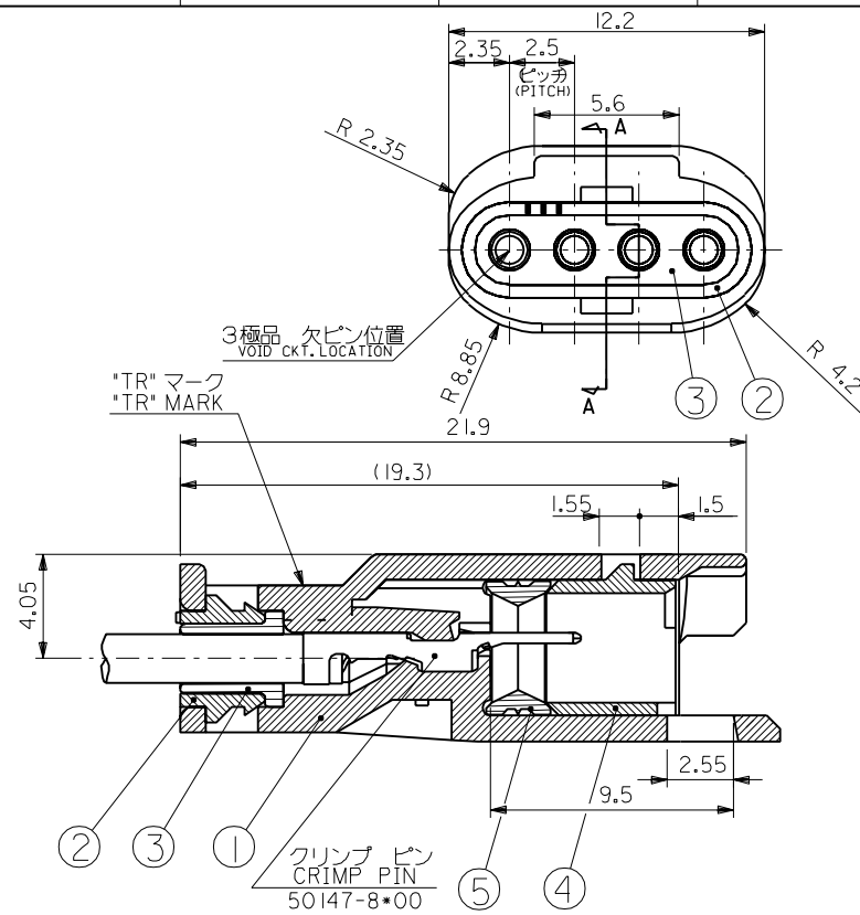
断面A-A (端子装着状態図) SECT.A-A(TERM.ASSEMBLY DRAWING)
