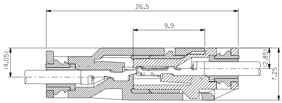
嵌合状態図 FULLY MATED CONDITION
