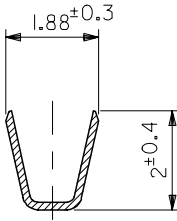
SECT. B-B
