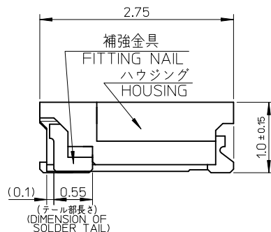
SECTION Y-Y
