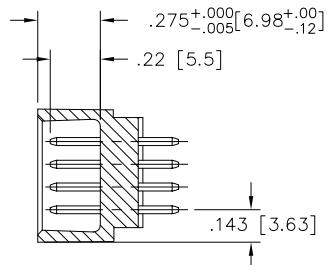
SECTION X-X
