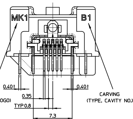
SECTION Z-Z
