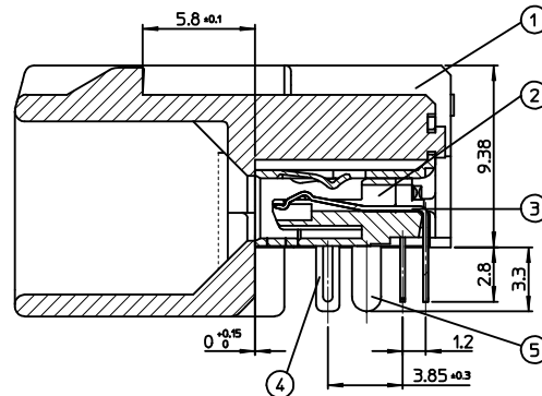
SECTION Z-Z
