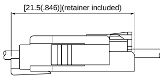
PAL Receptacle + PA Receptacle (Standard type)
