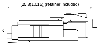
PAL Receptacle + PA Receptacle (Retainer mountable type)
