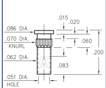
9393-0-15-XX-47-XX-10-0 Press-fit in .067 mounting hole.
