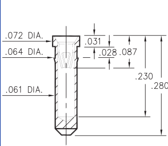
6857-0-15-XX-47-XX-10-0 Press-fit in .061 mounting hole.
