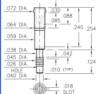
4614-0-31-XX-47-XX-04-0 Compliant press-fit in .040±.003 plated hole. For .060→.100 thick board.
