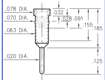
0400-0-15-XX-47-XX-04-0 Press-fit in .067 mounting hole.
