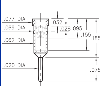
2400-0-15-XX-47-XX-04-0 Press-fit in .066 mounting hole.
