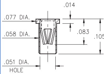
7305-0-15-XX-47-XX-10-0 Solder mount in .060 min. mounting hole Also available on 24mm wide carrier tape: 1,500 parts per 13" reel. Order as: 7305-0-57-XX-47-XX-10-0
