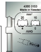
431 53 PortaCrimp Wire Ferrules - Insulated & Non-Insulated Die set for 6-4 AWG (16-25mm).
