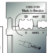
431 54 PortaCrimp Wire Ferrules - Insulated & Non-Insulated Die set for 2-1/0 AWG (35-50mm).
