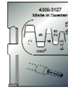
431 27 PortaCrimp Wire Ferrules - Insulated & Non-Insulated Die set for 24-8 AWG (0.25-10mm).
