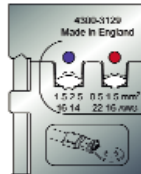
431 29 PortaCrimp Die Set For Red & Blue Insulated Terminals & Splices Die set for 22-14 AWG (0.5 - 2.5mm).
