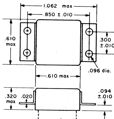
End Bracket
