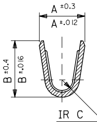
SECT. G-G
