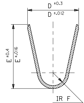
SECT. H-H
