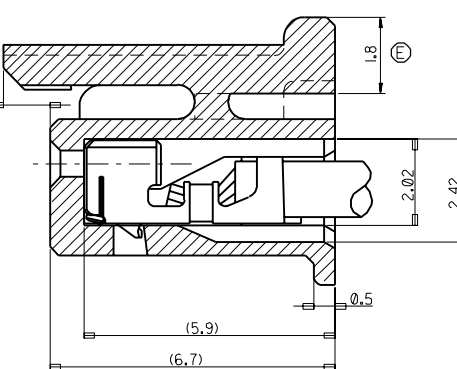
TERMINAL INSERTED DRAWING SCALE 2:1
