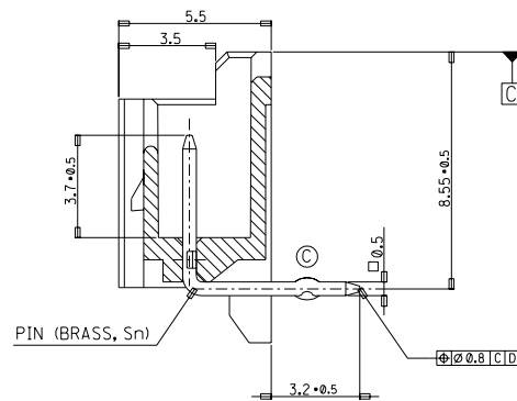
SECTION K-K'
