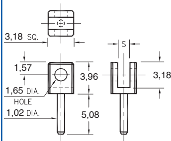
3620-X-32-XX-00-00-08-0 Board edge rivet mount
