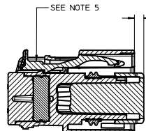
SECTION B-B SCALE 2:1 (RECEPTACLE INSERT SHOWN IN PRE-LOCK POSITION) SEE NOTE 2
