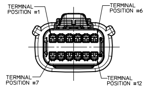
REAR VIEW (WIRE HARNESS SIDE)
