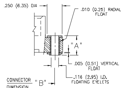
MOUNTING OPTION CODE x03
