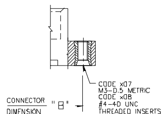
MOUNTING OPTION CODES x07 & x08
