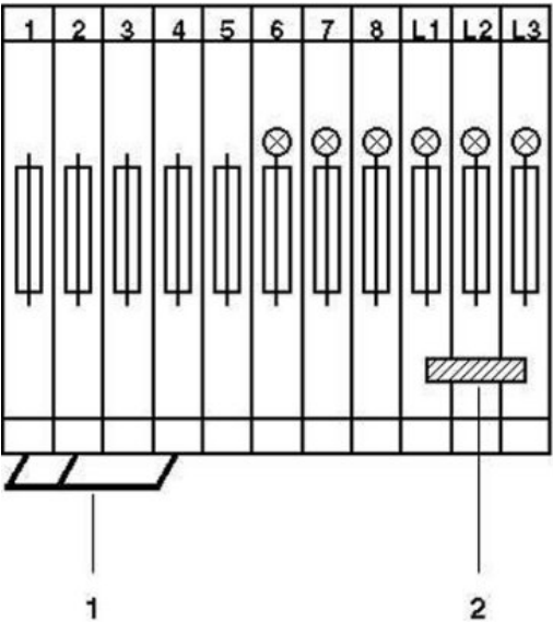
Circuit diagram
