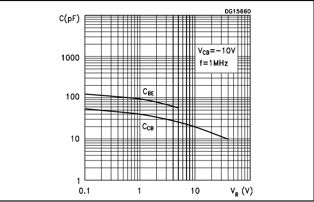
Figure 7. Capacitance
