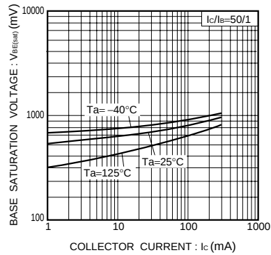
Fig.10 Base-emitter saturation voltage vs. collector current (III)
