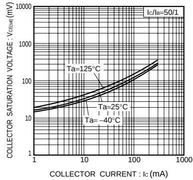
Fig.7 Collector-emitter saturation voltage vs. collector current (III)
