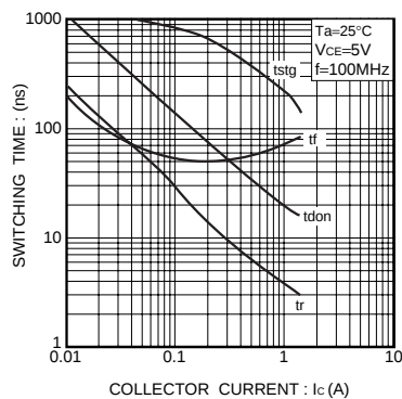
Fig.7 Switching time
