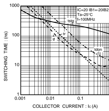
Fig.6 Switching time
