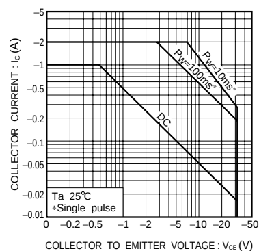
Fig.9 Safe operation area (2SB1132)
