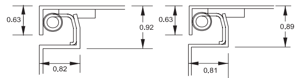
Cross Section of 14 Gauge Body & Door
