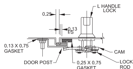
Cross Section of Handle Channel Detail
