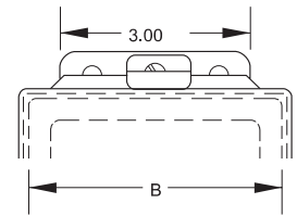
Mounting Foot Detail When B=4
