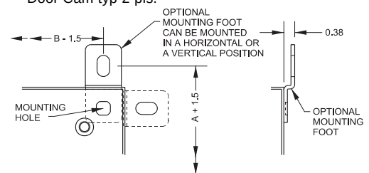
Mounting Detail
