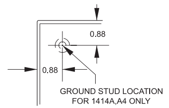
Ground stud location for 1414A, 1414A4 only
