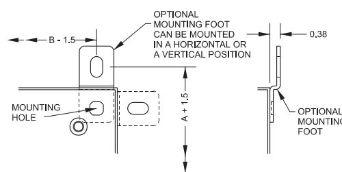
Mounting Detail
