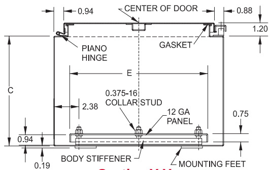
Section Y-Y
