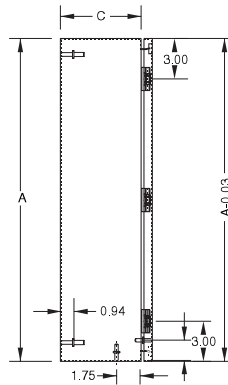
Side View Hinge Side
