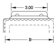
Mounting Foot Detail When B=4
