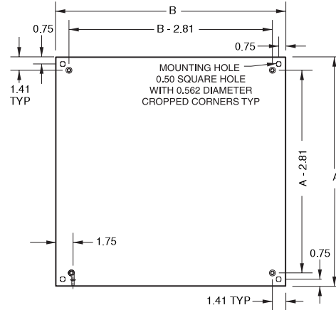
Front Section Door & Body Flange Removed
