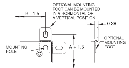
Mounting Detail Door & Body Flange Removed
