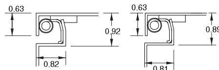
Cross Section of 14 gauge Body & Door
