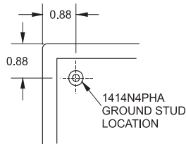
Ground stud location for 1414N4PHA
