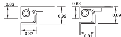
Cross Section of 14 gauge Body & Door
