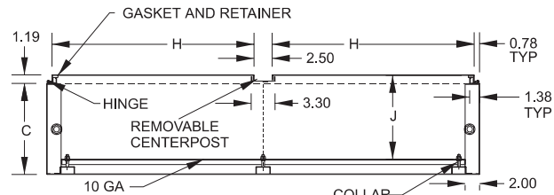
Section X-X
