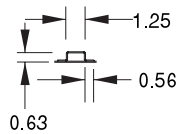
Section Z-Z (Except 1422VX12 & 1422WW12)
