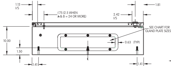
End View with Gland Plate
