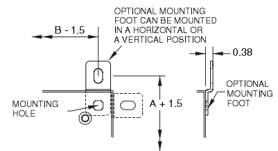
Mounting Detail Door & Body Flange Removed
