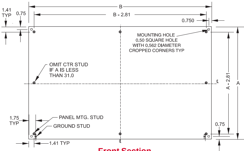
Front Section
