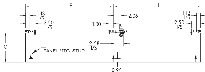
End View
