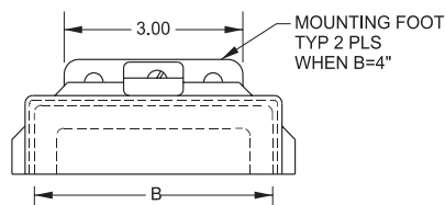
Mounting Foot Detail When B=4
