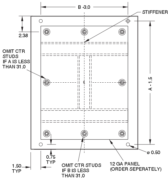
Section Y-Y
