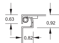
Cross Section of 14 gauge Body & Door
