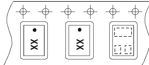
DFN1006-3 Taping orientation
