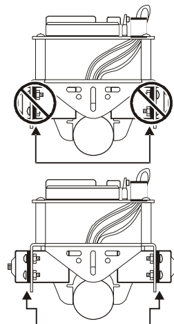
Servo mounting tabs are outside of chassis
