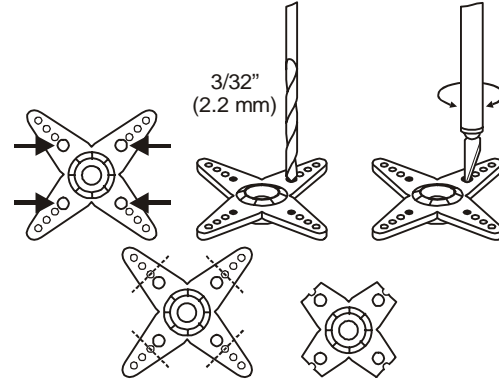
Enlarge Inner Holes if using Standard Servo Horns
