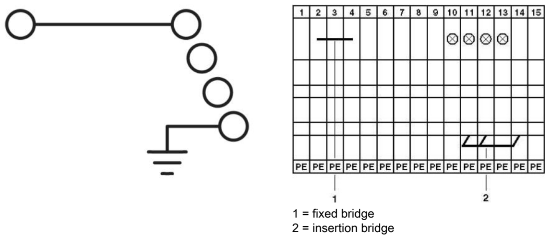
Circuit diagram
