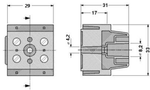
Dimensioned drawing
