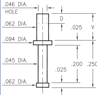
2329-X-00-XX-00-00-07-0 Swage mount in .067 hole
