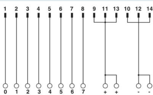
Connection scheme: FLKM 14/PLC
