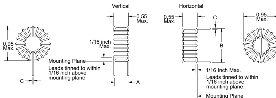
Dimensions: Inches
