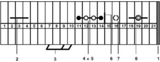
Circuit diagram
