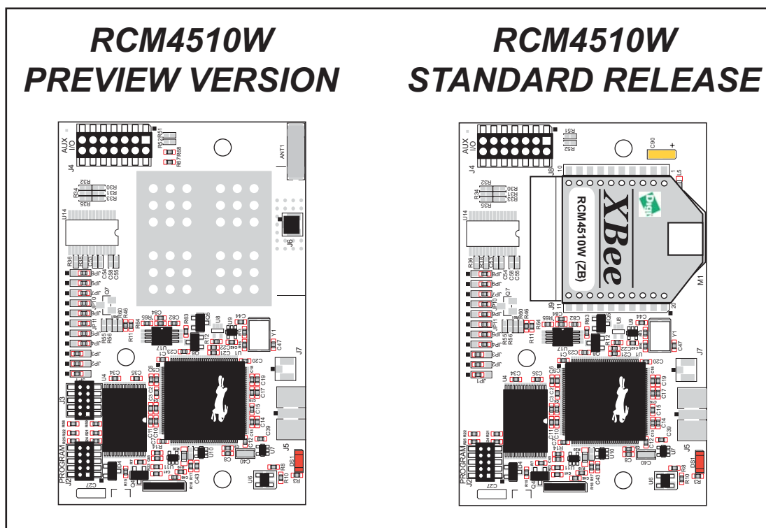
Figure 1. RCM4510W Versions
