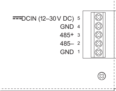
Figure 3-18. RS-485 Signals
