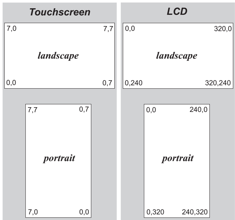
Figure 3-8. Coordinate Systems (row, column)
