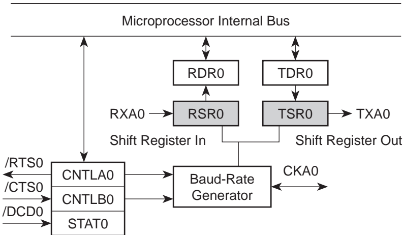
Figure 3-21. Z180 Serial Channel 0
