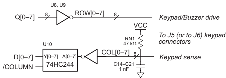
Figure 3-10. Block Diagram of OP7100 Keypad Interface
