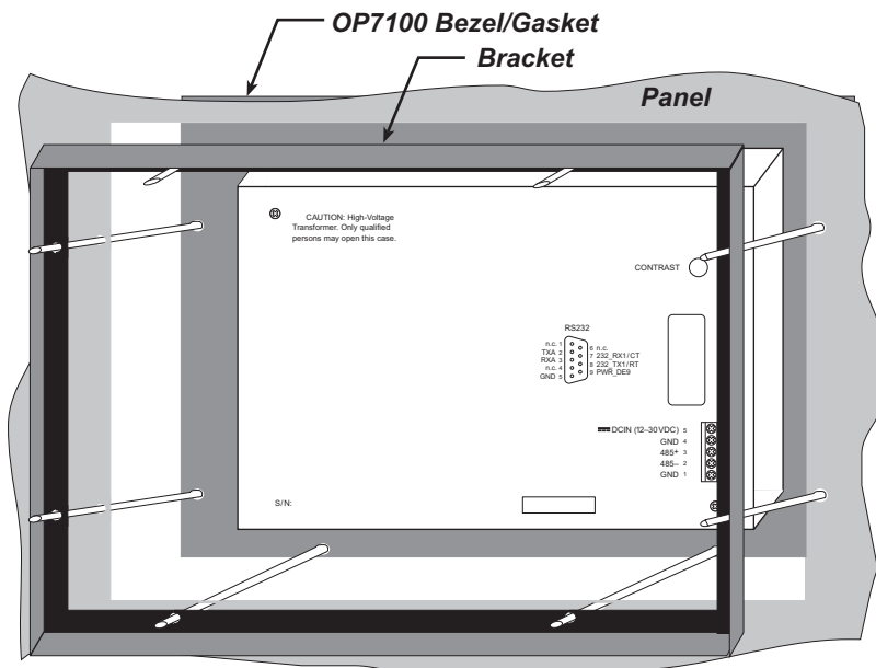
Figure 6-3. Strengthening Bracket
