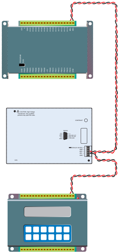
Figure 3-19. RS-485 Network
