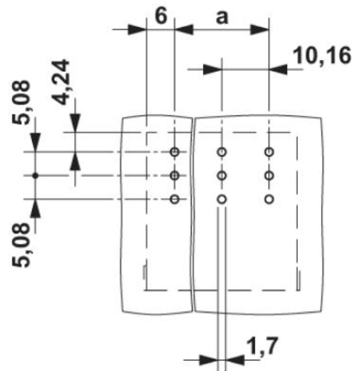
Drilling diagram
